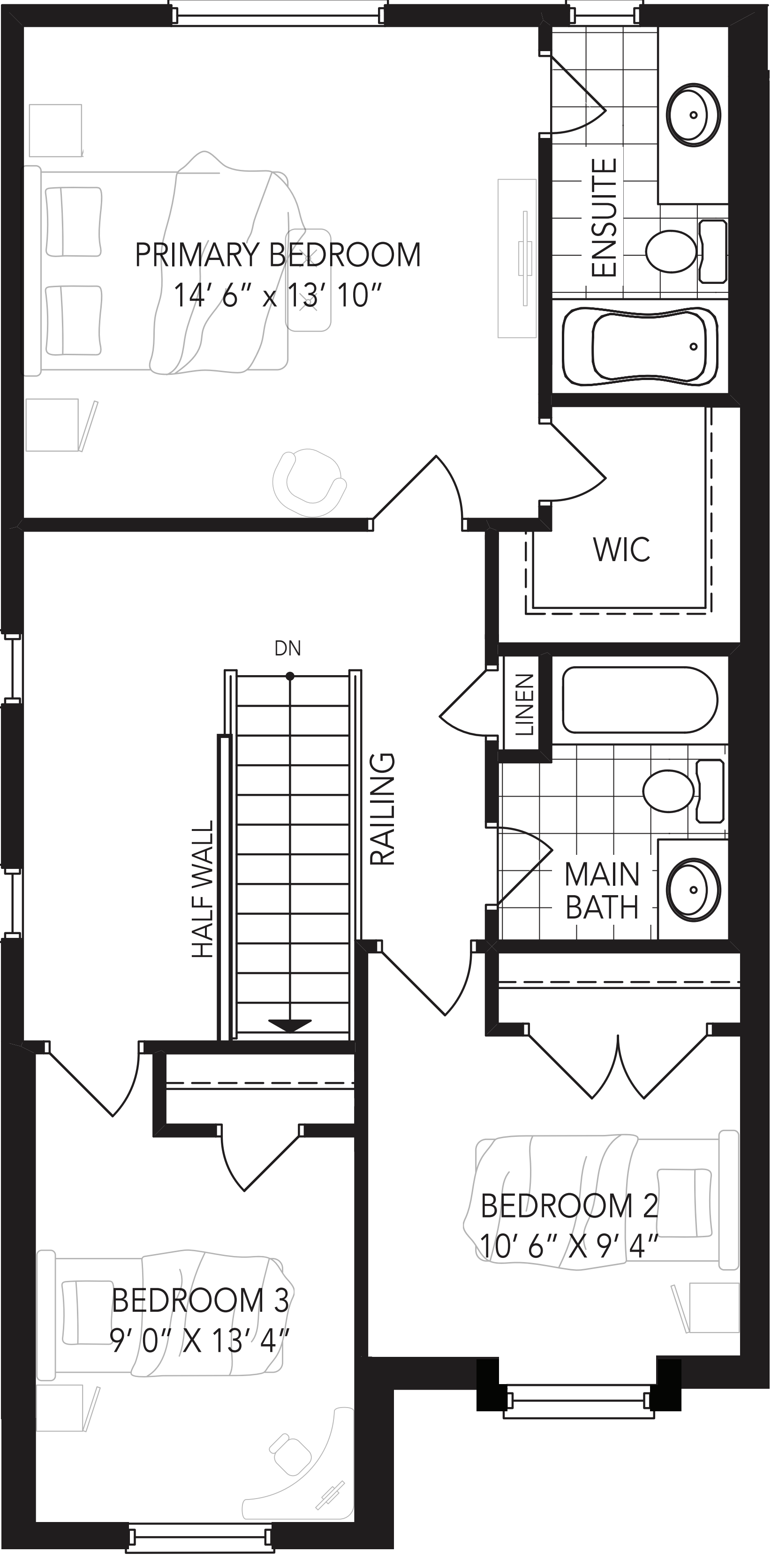
Second Floor
