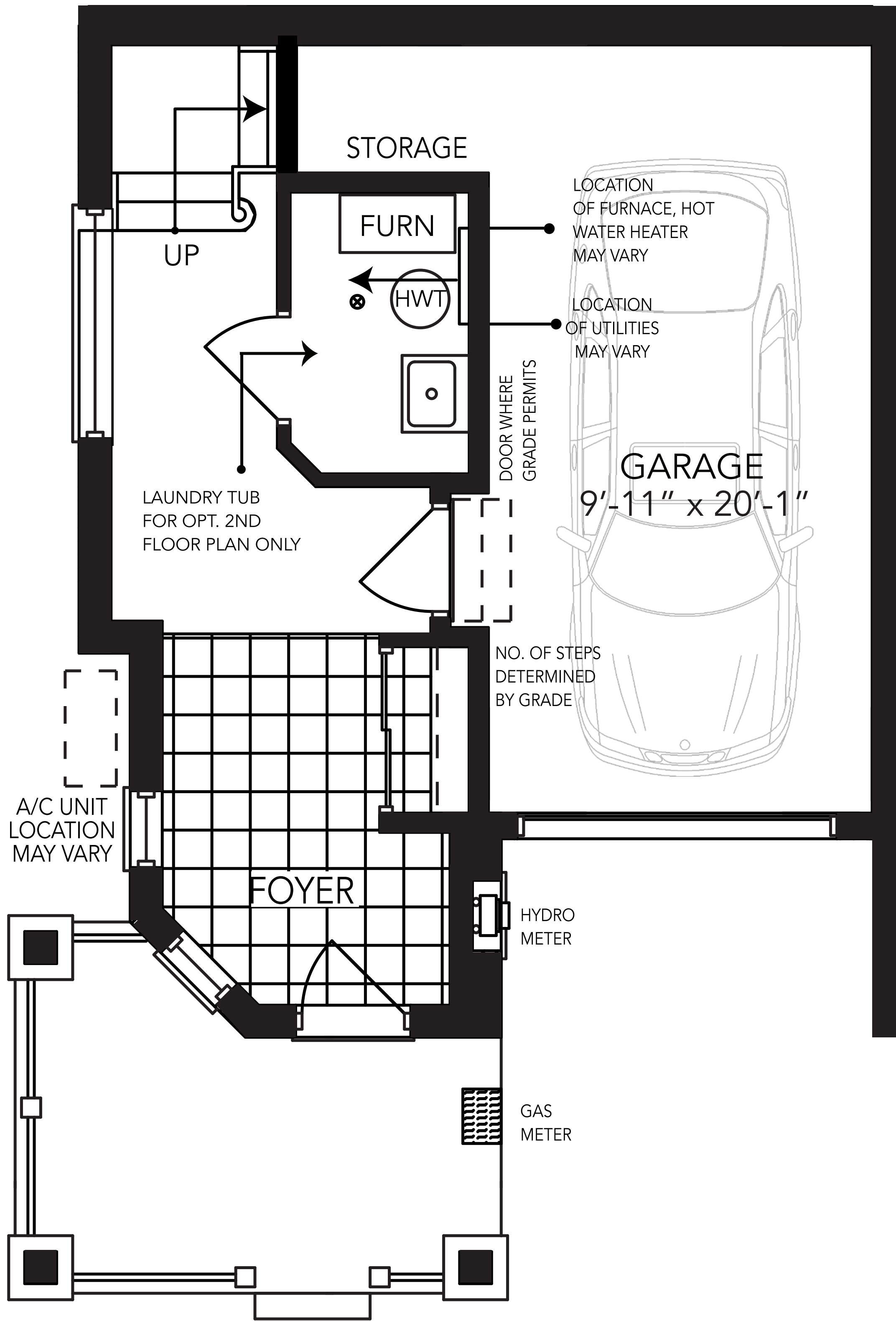
Main Floor
