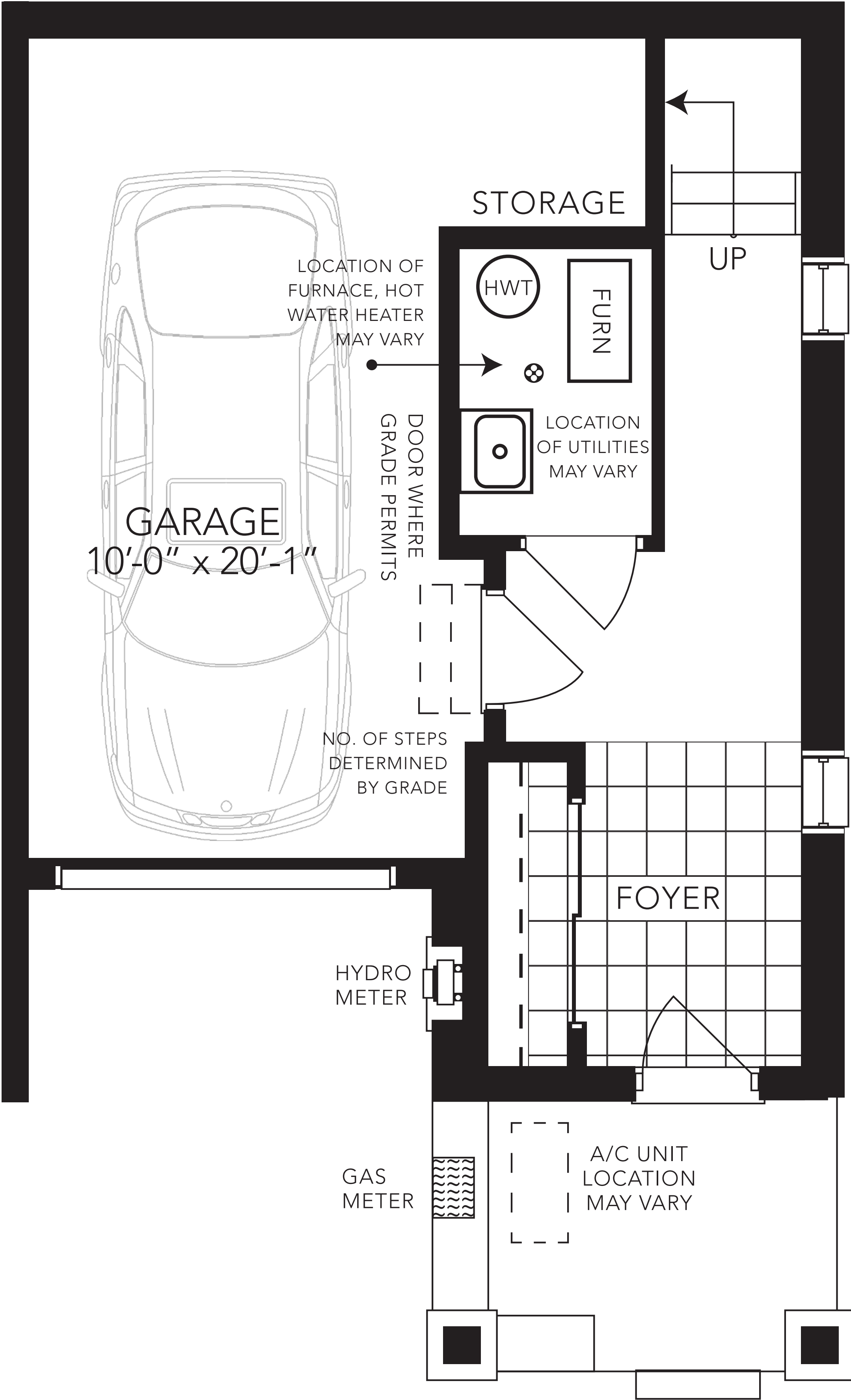
Main Floor
